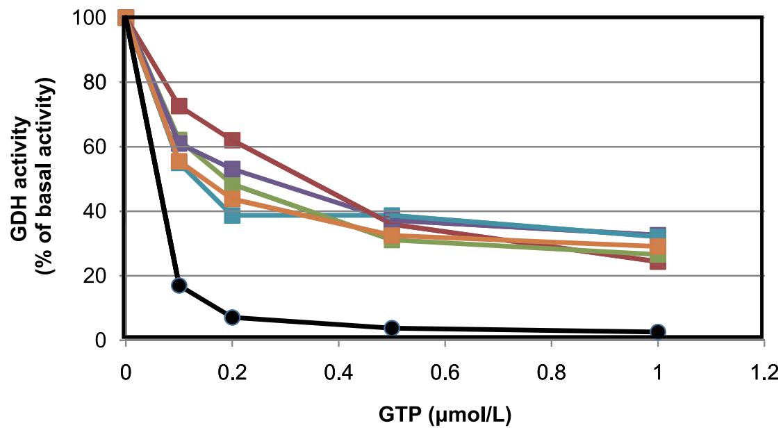
Figure 1. Effects of GTP on glutamate dehydrogenase (GDH) activity in lymphoblasts of Patients 11, 1-4, and control subjects. Orange line, Patient 11; red, Patient 1; green, Patient 2; purple, Patient 3; blue, Patient 4; and black, controls (n=5).
