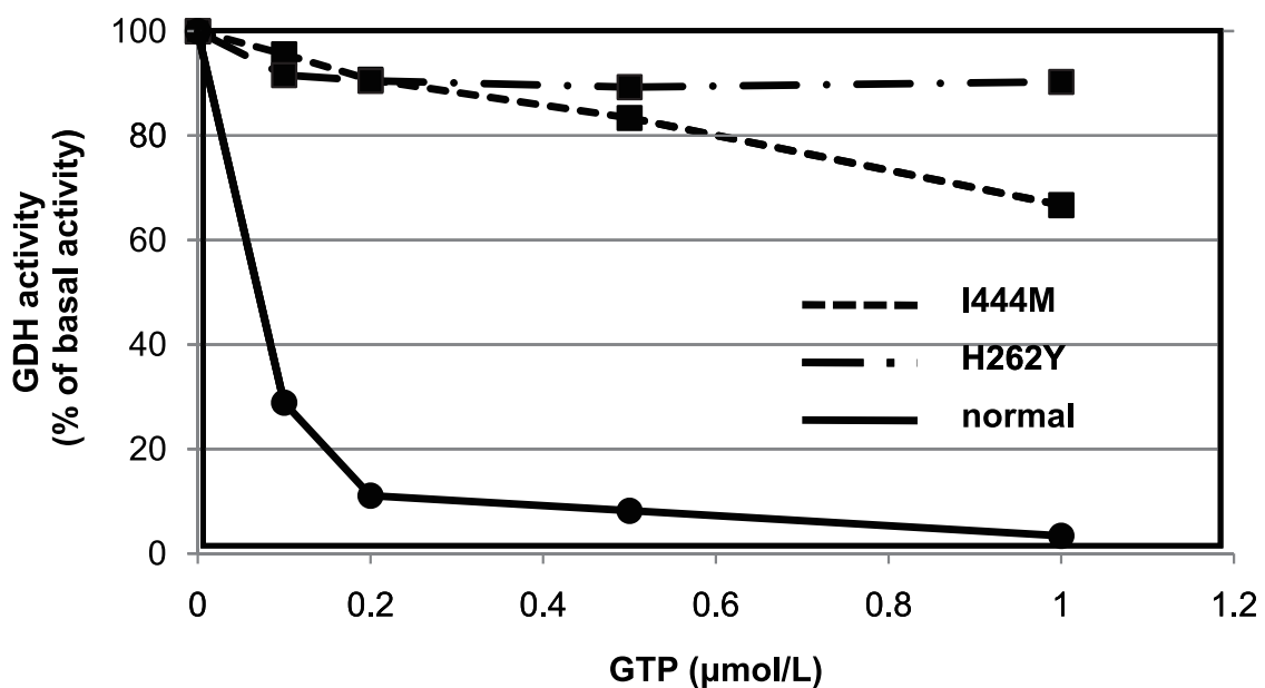
Figure 2. Effects of GTP on glutamate dehydrogenase (GDH) activity in COS cells transfected with normal or the indicated mutant cDNAs constructs by expression analysis.
