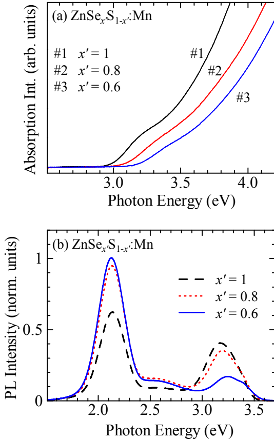
Figure 2. (a) Absorption and (b) PL spectra of ZnSe _x S _{1-x} :Mn QDs, where x' = 0.6, 0.8 , and 1, synthesized with the reaction time of 15 min.
