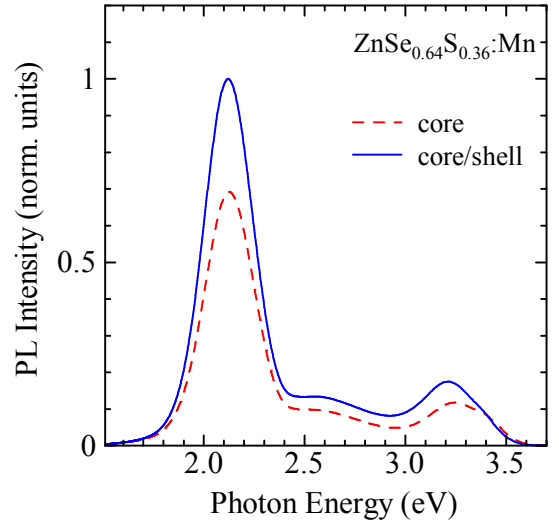
Figure 4. PL spectra of ZnSe _{0.64} S _{0.36} :Mn core QDs (dashed curve) and ZnSe _{0.64} S _{0.36} :Mn/ZnS core/shell QDs (solid curve).
