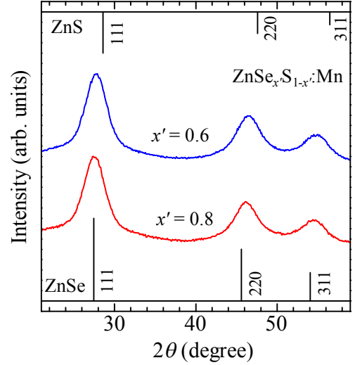
Figure 3. XRD patterns of ZnSe _x S _{1-x} :Mn QDs, where x' = 0.6 and 0.8 (JCPDS Card No. 80-0021 for ZnSe and 05-0566 for ZnS).
