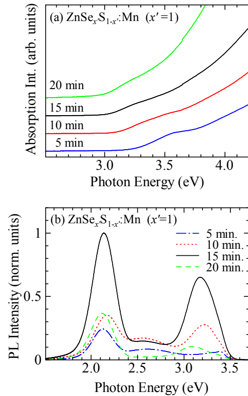
Figure 1. (a) Absorption and (b) PL spectra of ZnSe:Mn QDs synthesized with reaction times of 5, 10, 15, and 20 min.
