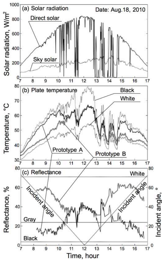
Fig. 6 The results of the exposure test: (a) The amount of direct and sky solar radiations measured by a pyranometer tilted at 22^{\circ} towards the south (b) Measured plate temperatures (c) The solar reflectances of the prototypes calculated using the solar reflectance of white, gray, and black plates as references
