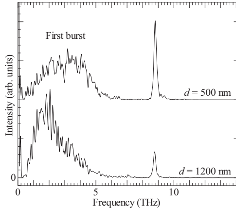
Figure 3. Fourier power spectra of the terahertz waveforms of the i -GaAs( d nm)/ n -GaAs structures. The time window is the same as the scan range: [-2.0 ps, 8.0 ps]. The band peaking at 8.8 THz originates from the coherent GaAs LO phonon.
