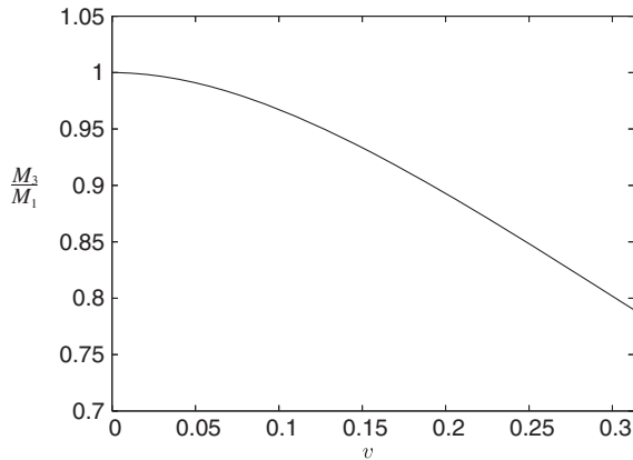
FIG. 13. The mass parameter M_3 in the case of r_{d2} = r_{d1} = 1.00001 \times 2M_1 is depicted as a function of v .
