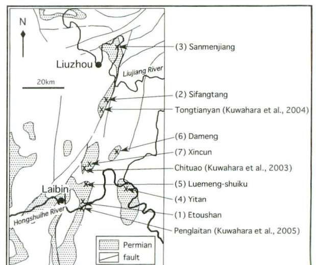
Fig. 2 Distribution of the Permian and location of study sections in the Laibin - Liuzhou area of the central Guangxi (after Bureau of Geological and Mineral Resources of Guangxi Zhuang Autonomous Region, 2002).
