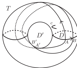
Fig.2. Hopf fibration
