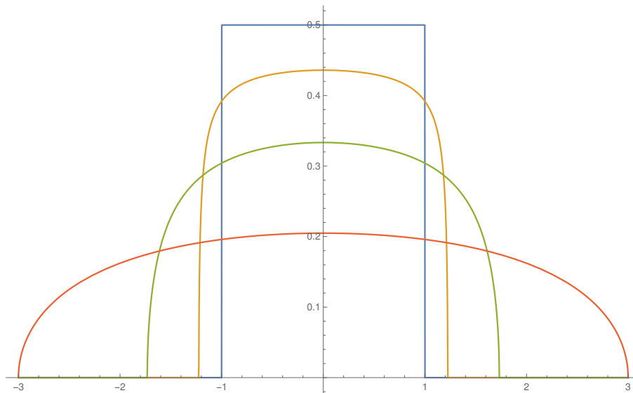
FIGURE 4. The function \tilde{\rho}(x) for c = 1 (blue), c = \frac{3}{2} (orange), c = 3 (green) and c = 9 (red).
